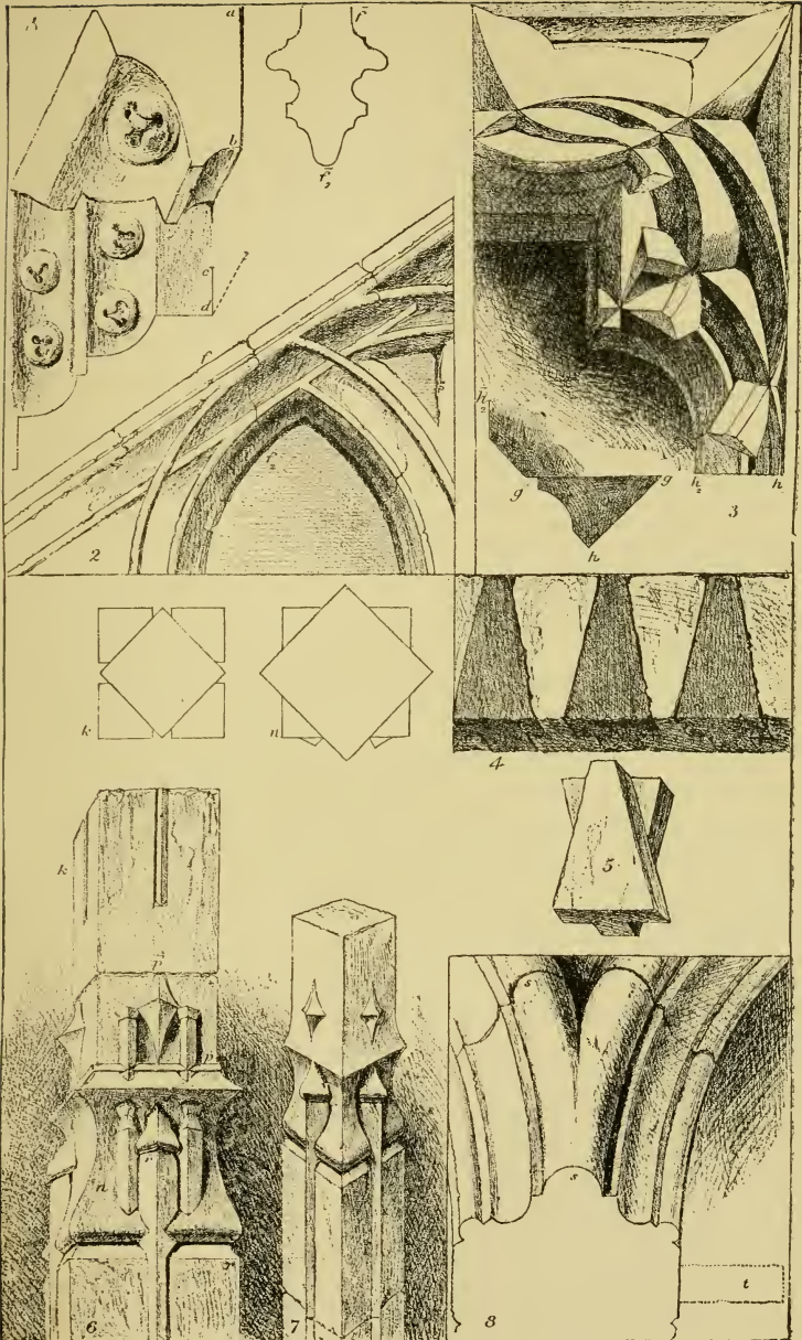
PLATE IV.—(Page 66—Vol. V.) INTERSECTIONAL MOULDINGS.
