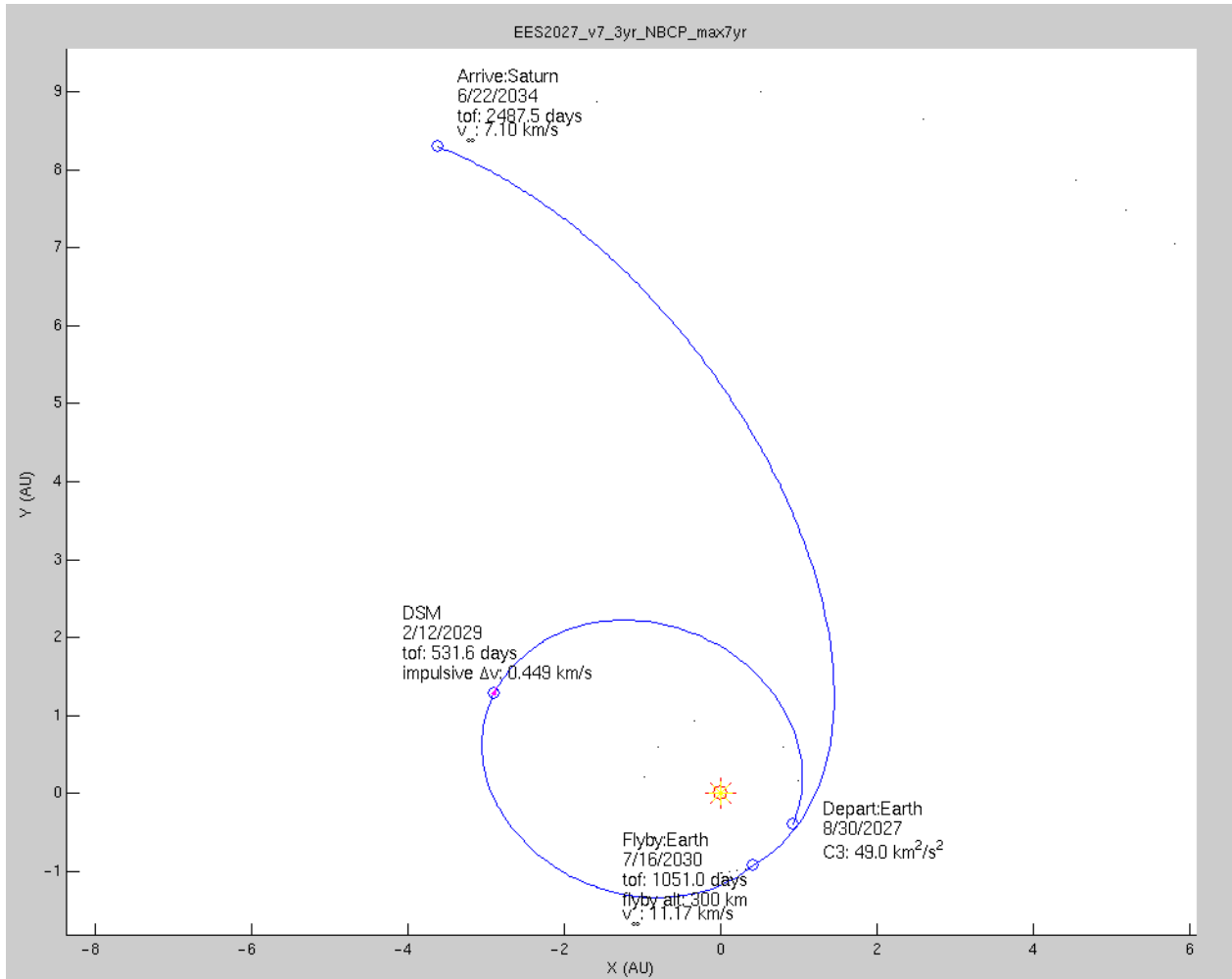
Figure 3-1. Baseline Trajectory
